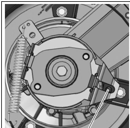
Align anti-rotation arm with shoulder bolt bracket here.
