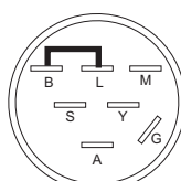
RUN
