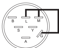
OFF
