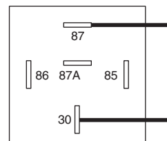
ENERGIZED
