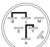
RUN / LIGHT
